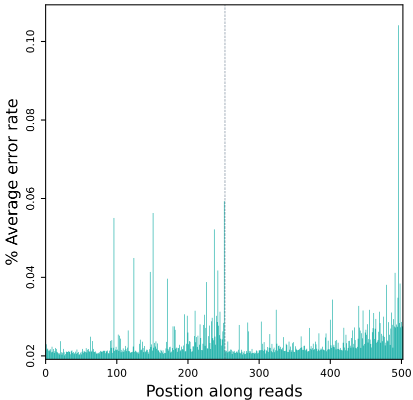
Error rate distribution along reads (R10907)
